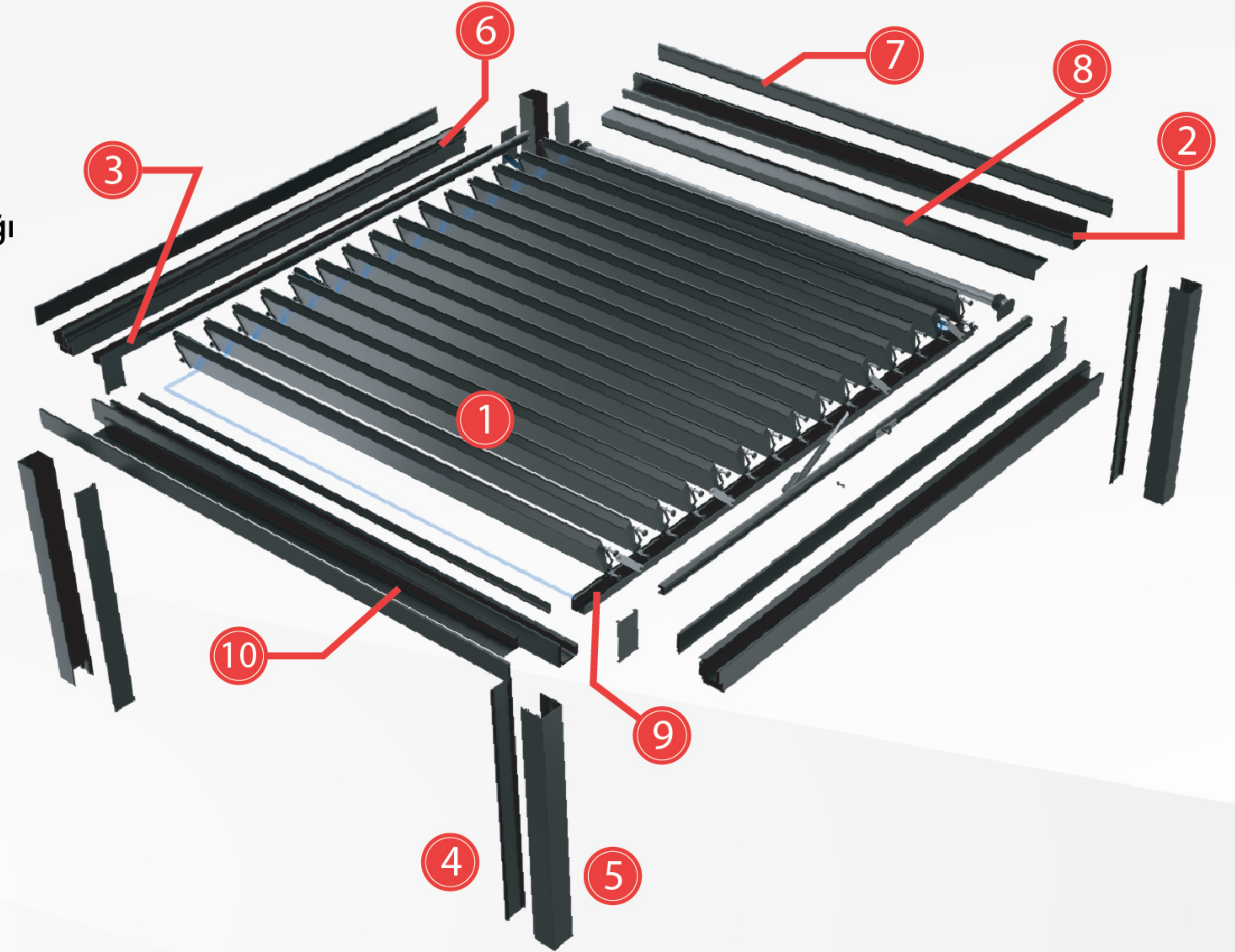
4614 Movina İç Oluk Movina Inner Gutter 1,336 kg/m
